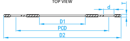
CROSS SECTIONAL VIEW
